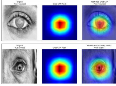
Fig. 9: Grad-CAM visualizations highlighting discriminative regions.
