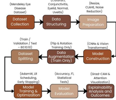
Fig. 1: Overall workflow of the proposed eye disease classification framework.
