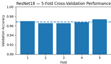
Fig. 7: 5-fold cross-validation validation accuracy across folds (ResNet18).
