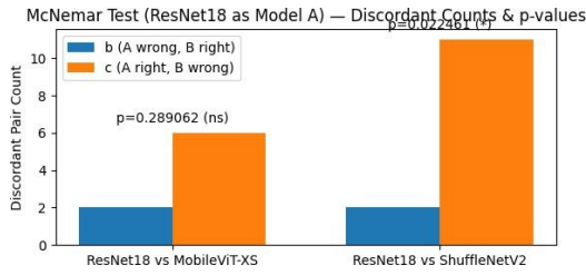
Fig. 6: McNemar paired test to evaluate the statistical significance of the best model.
