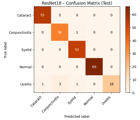
Fig. 5: Confusion Matrix for best performing model (ResNet-18).
