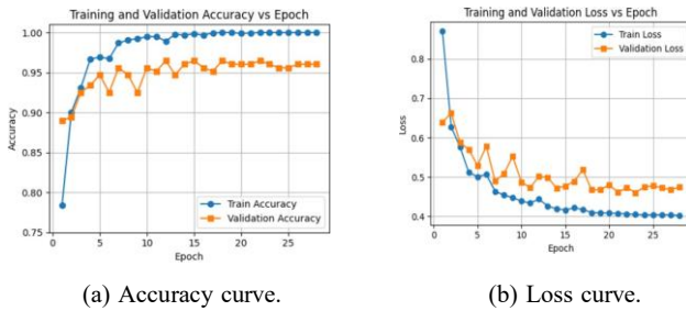
Fig. 4: Training and validation learning curves
